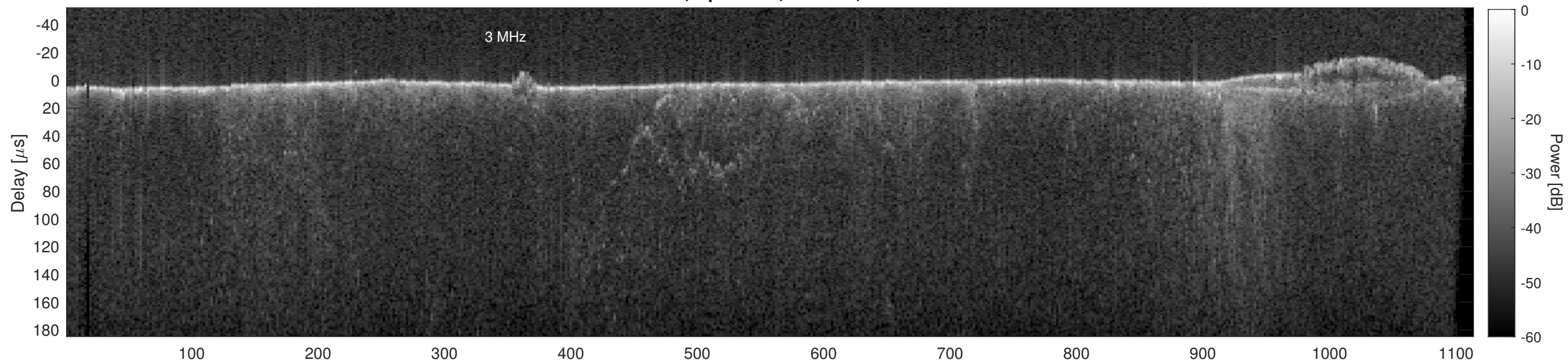
Orbit 18407, Cluttergram
