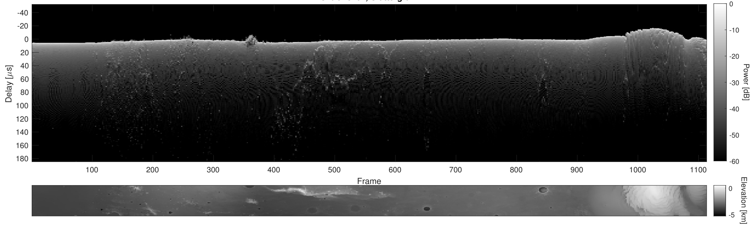
Orbit 18407, Cluttergram
