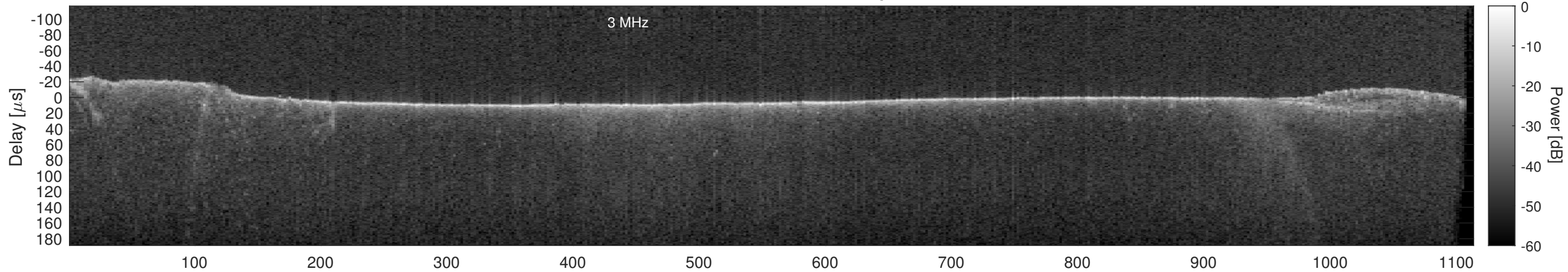
Orbit 18411, Cluttergram
