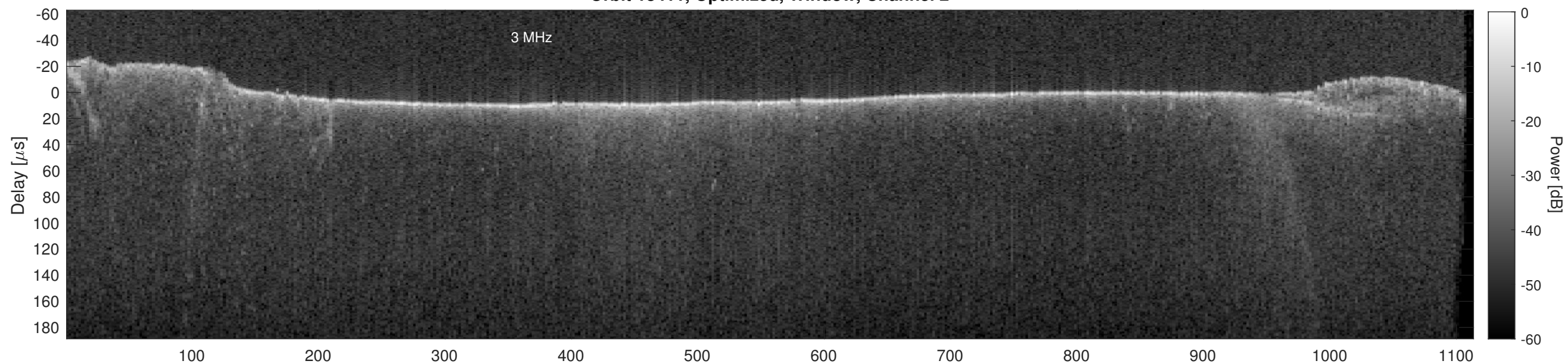
Orbit 18411, Cluttergram
