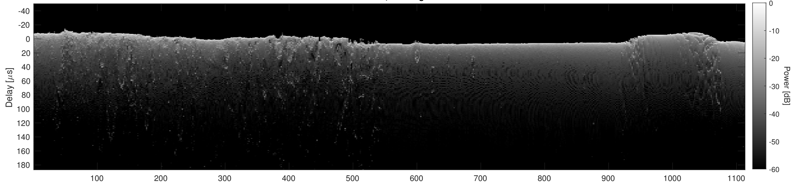
Orbit 18412, Cluttergram
