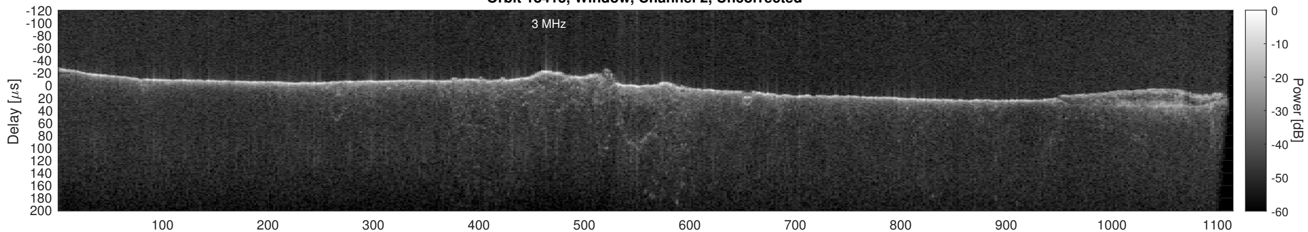
Orbit 18413, Window, Channel 2, Chapman
