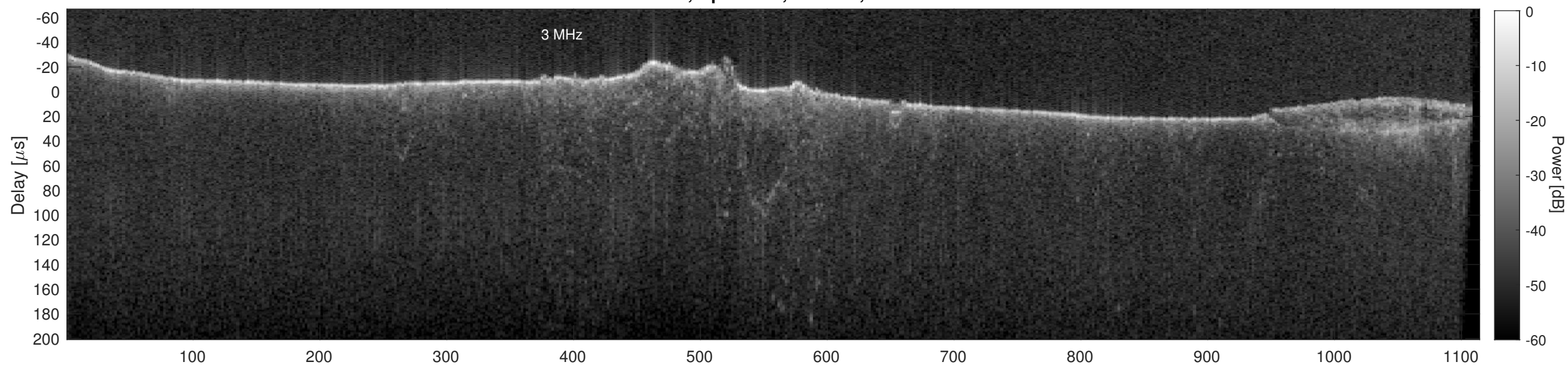
Orbit 18413, Cluttergram
