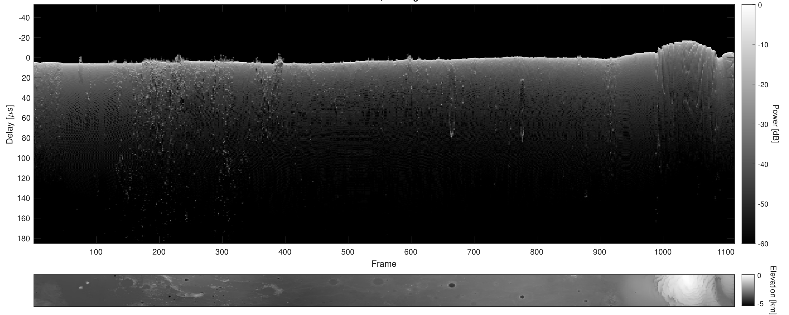
Orbit 18414, Cluttergram
