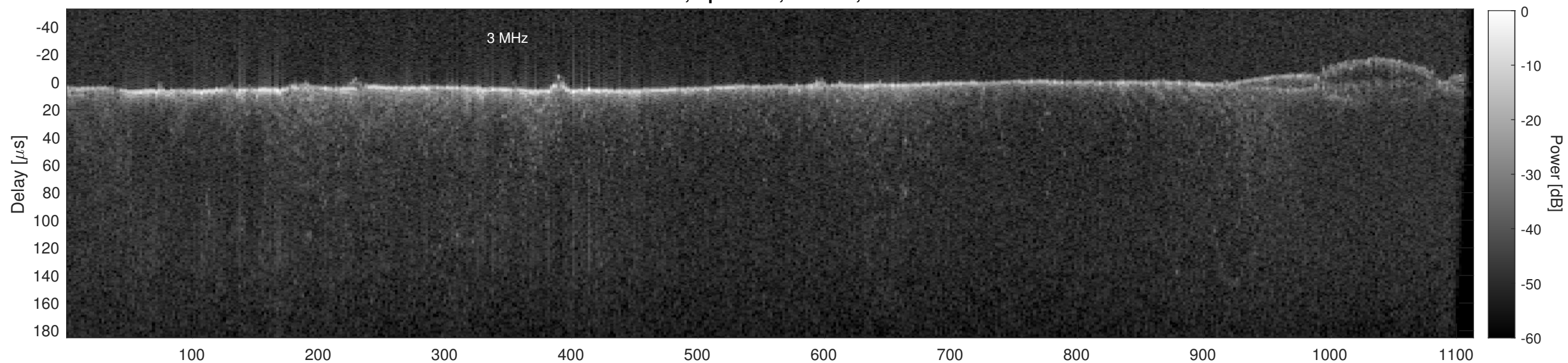
Orbit 18414, Cluttergram
