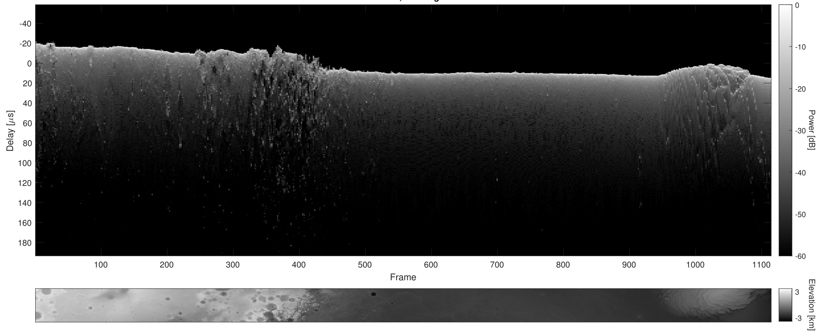
Orbit 18415, Cluttergram
