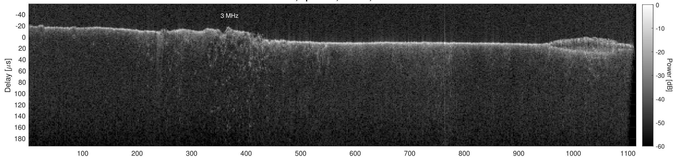
Orbit 18415, Cluttergram
