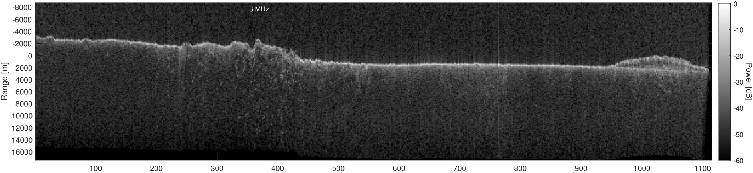
Orbit 18415, Depth-Corrected Cluttergram
