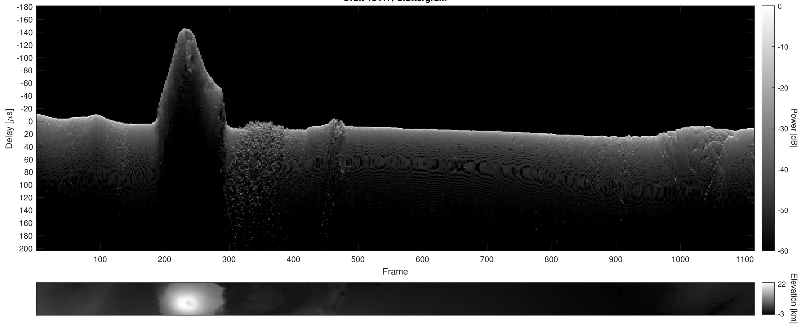
Orbit 18417, Cluttergram
