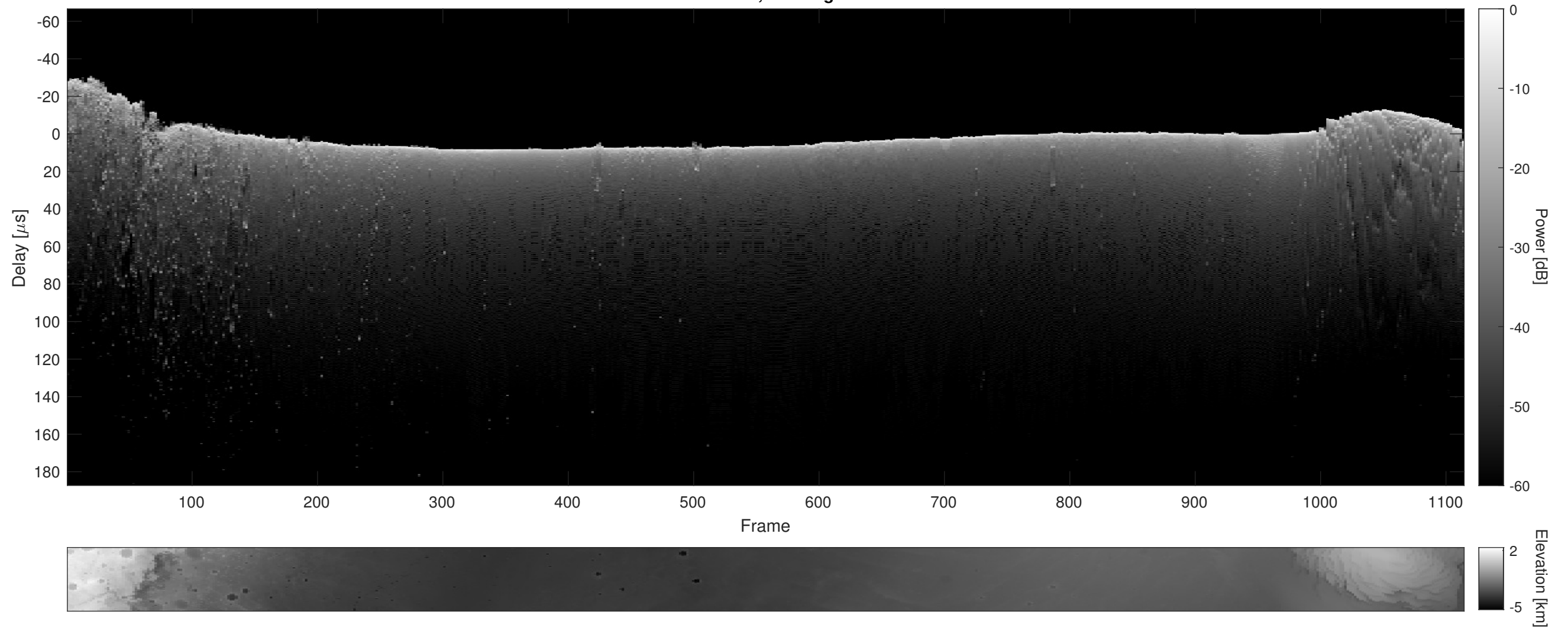
Orbit 18418, Cluttergram
