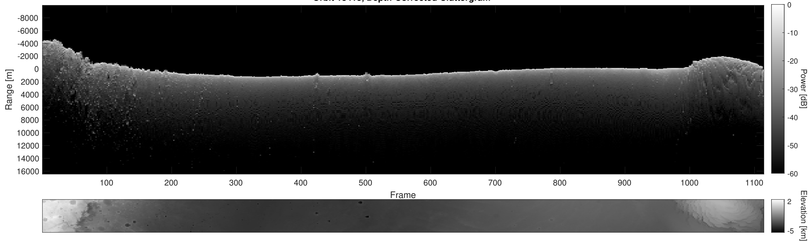
Orbit 18418, Depth-Corrected Cluttergram
