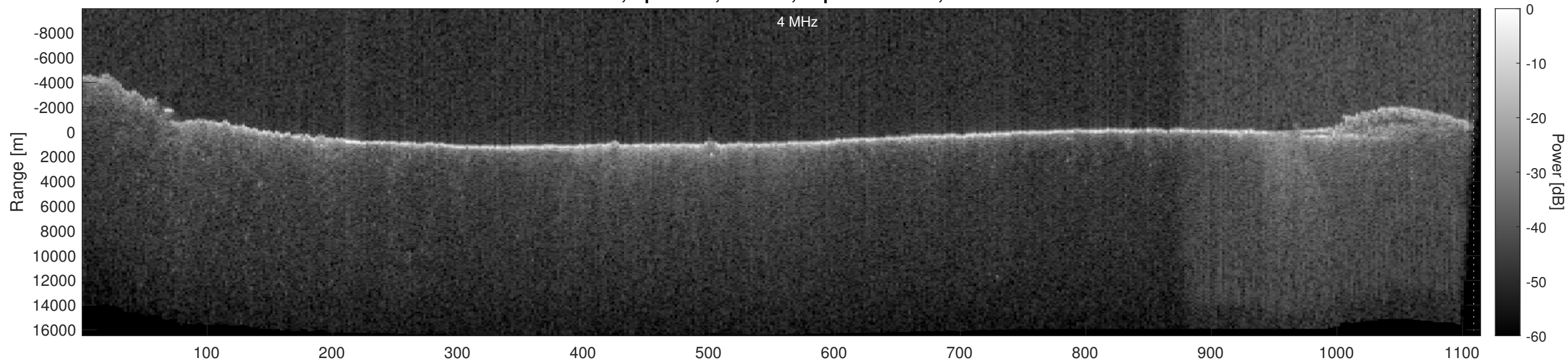
Orbit 18418, Optimized, Window, Depth-Corrected, Channel 2
