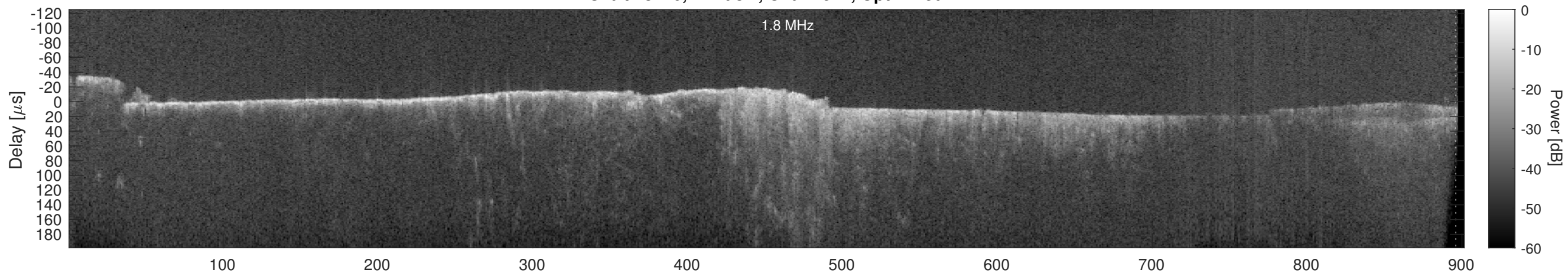
Orbit 18420, Cluttergram
