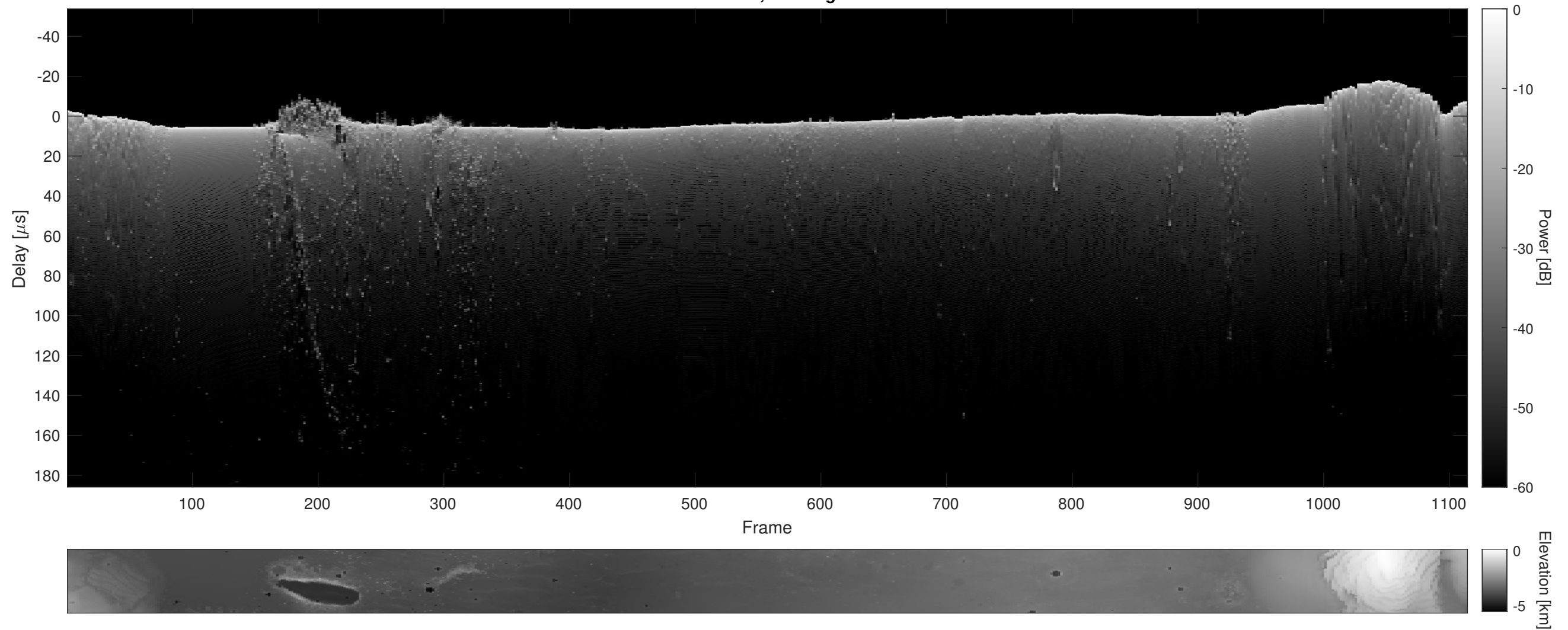
Orbit 18421, Cluttergram
