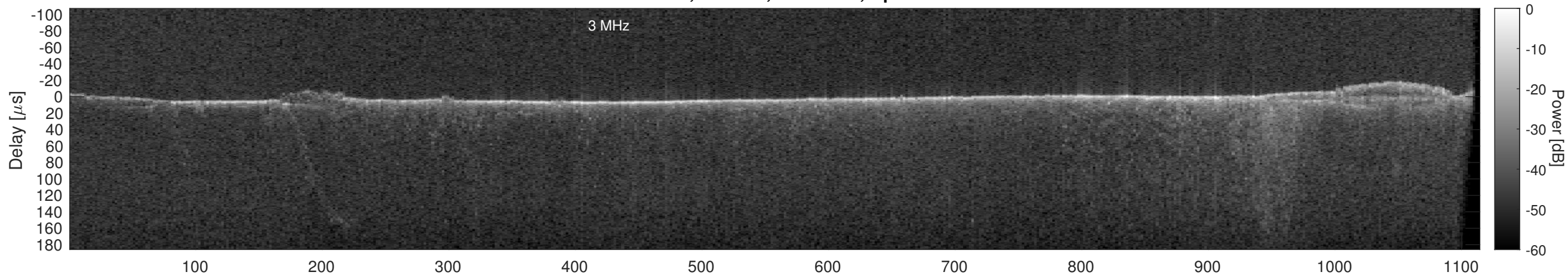
Orbit 18421, Cluttergram
