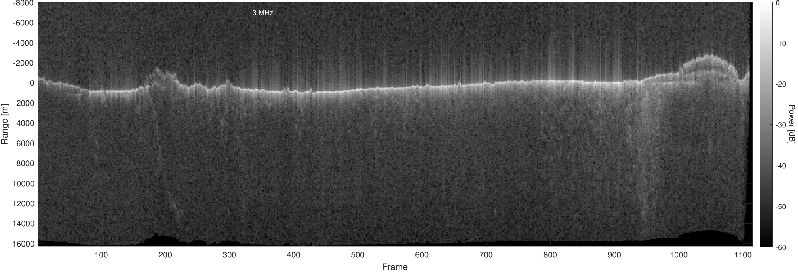
Orbit 18421, Optimized, No Window, Depth-Corrected, Channel 2
