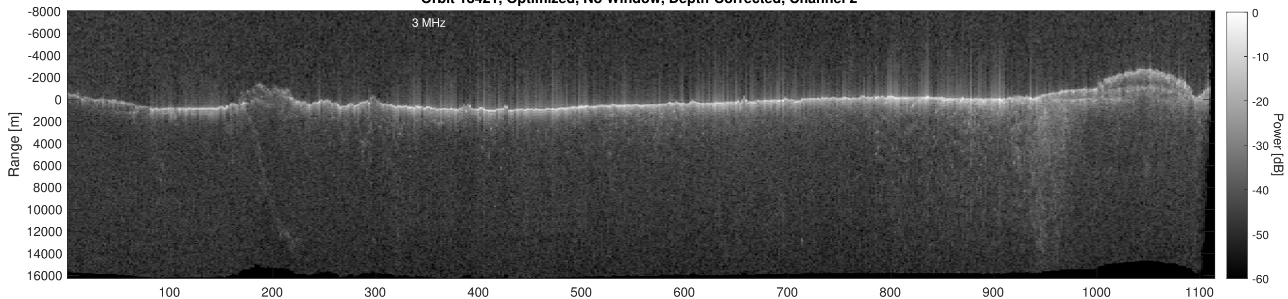
Orbit 18421, Depth-Corrected Cluttergram
