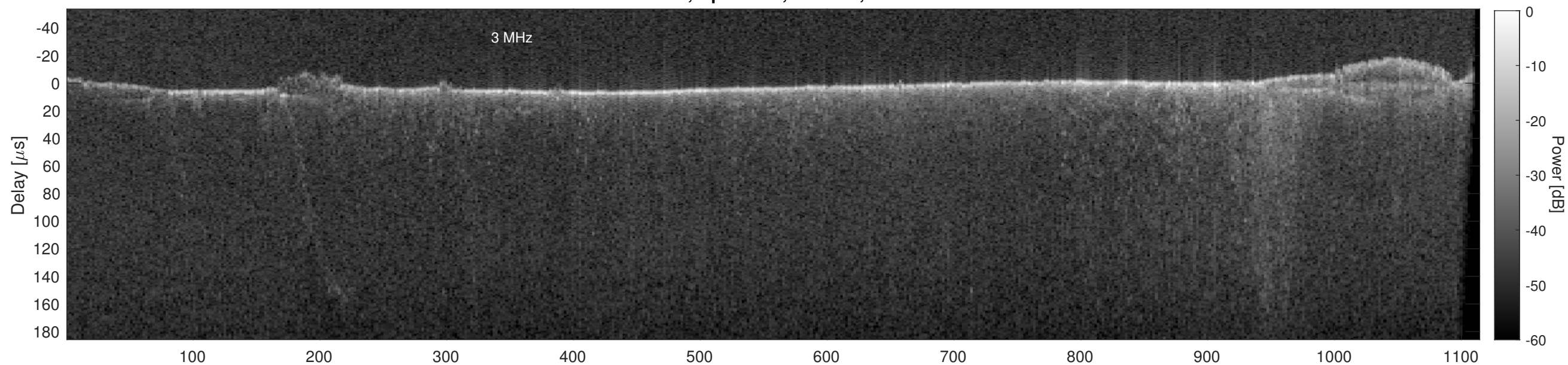
Orbit 18421, Cluttergram
