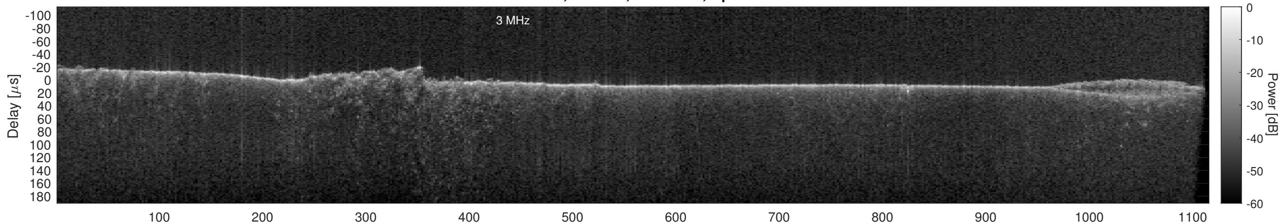
Orbit 18422, Cluttergram
