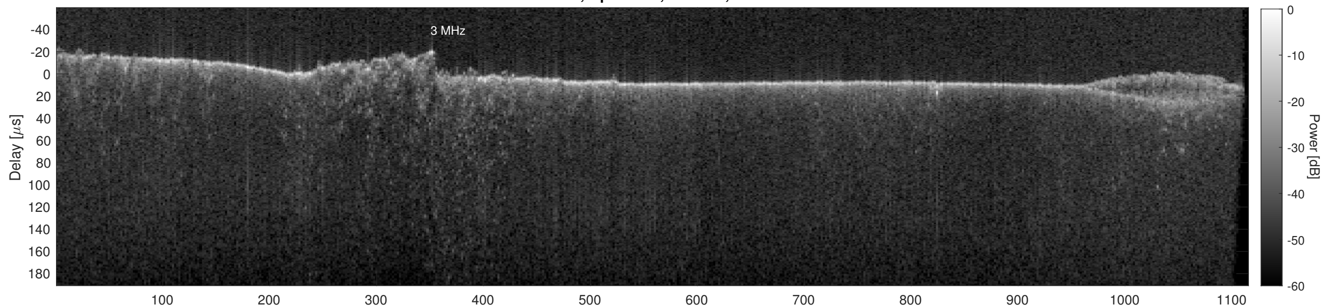
Orbit 18422, Cluttergram
