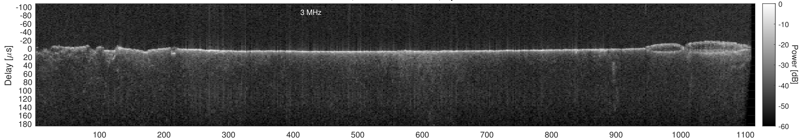
Orbit 18423, Cluttergram
