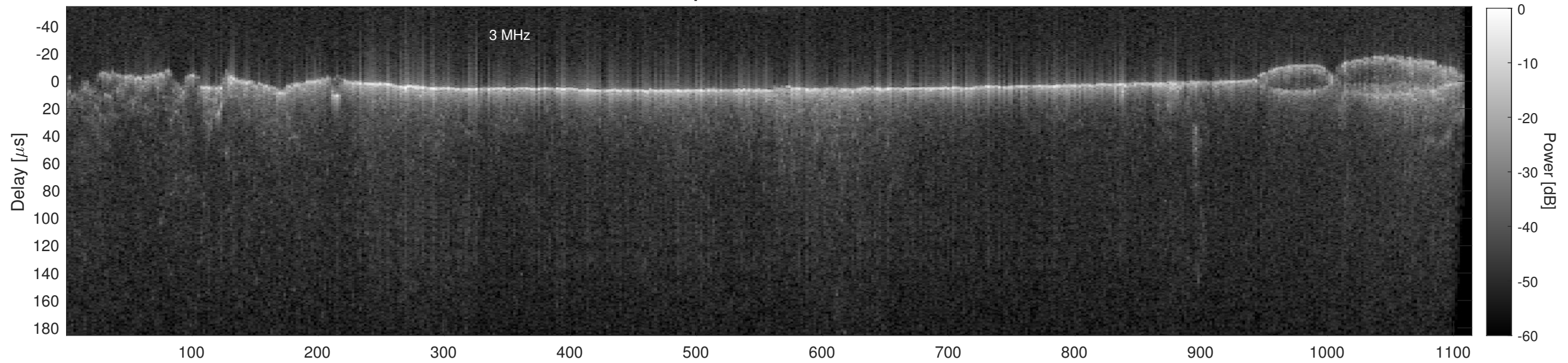
Orbit 18423, Cluttergram
