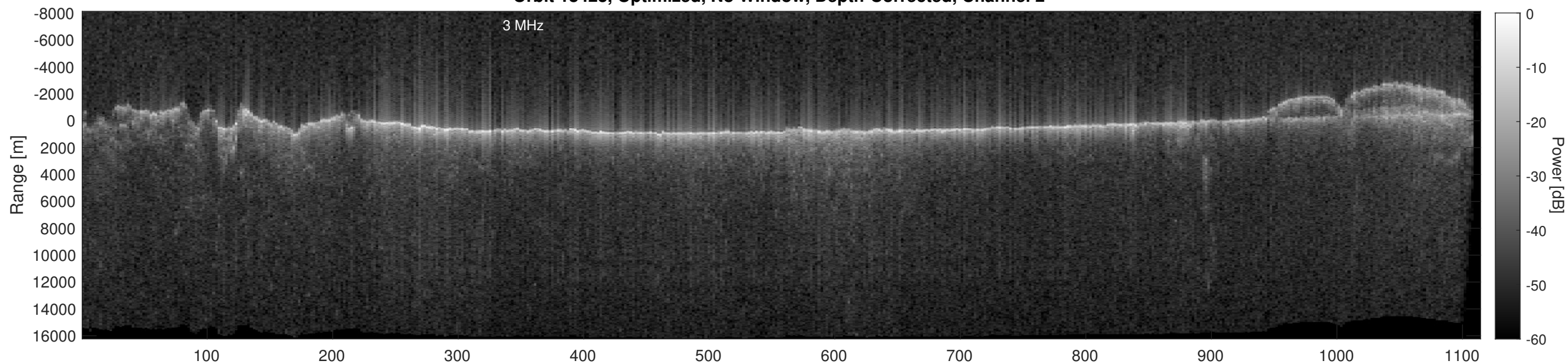
Orbit 18423, Depth-Corrected Cluttergram
