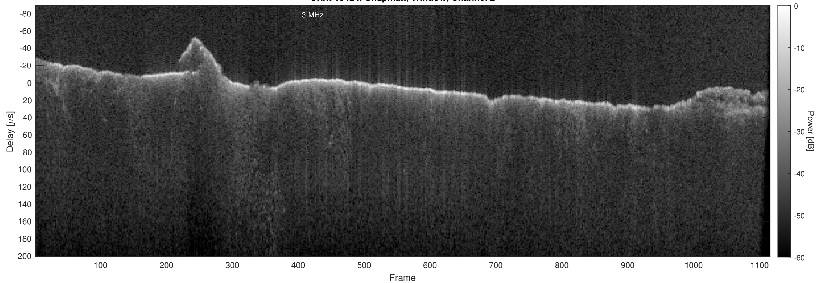
Orbit 18424, Chapman, Window, Channel 2
