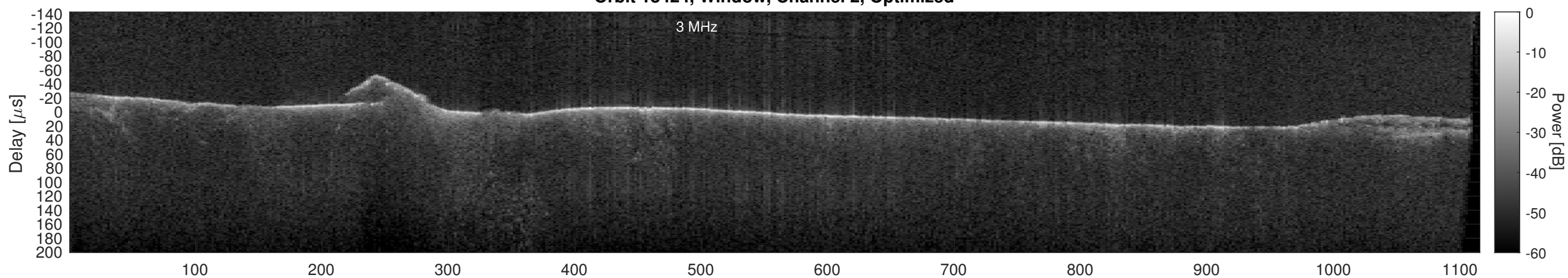
Orbit 18424, Cluttergram
