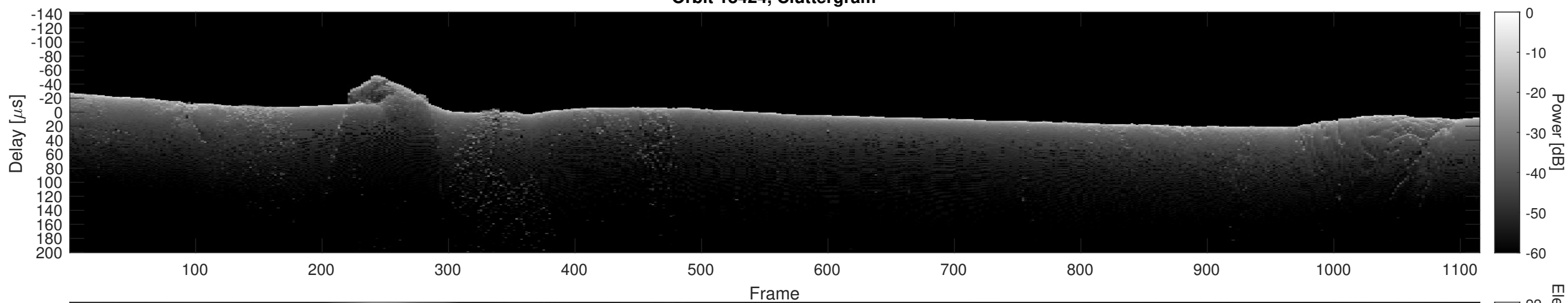
Orbit 18424, Cluttergram
