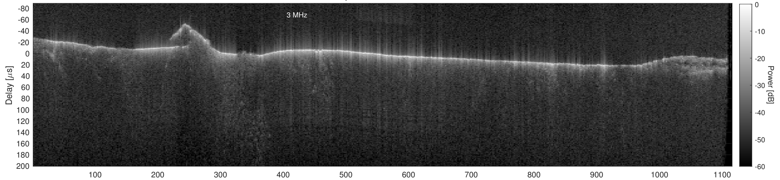
Orbit 18424, Cluttergram
