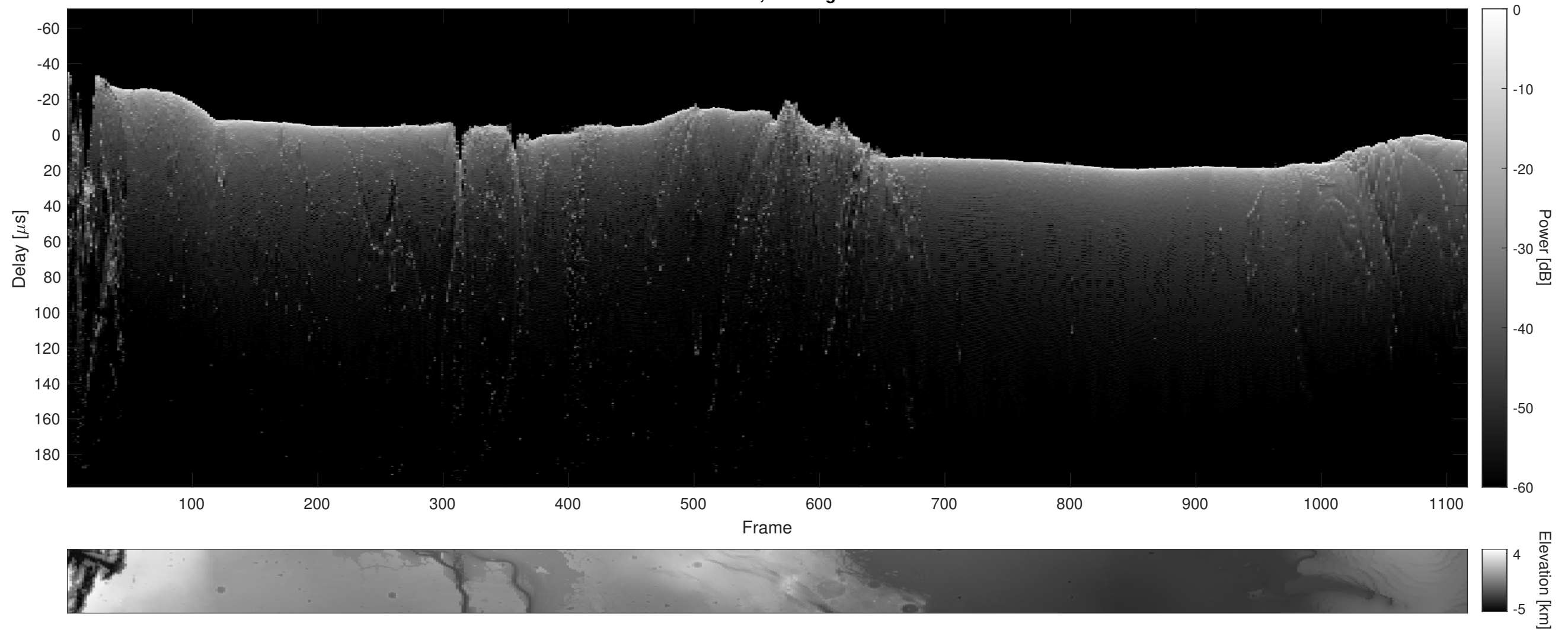
Orbit 18434, Cluttergram
