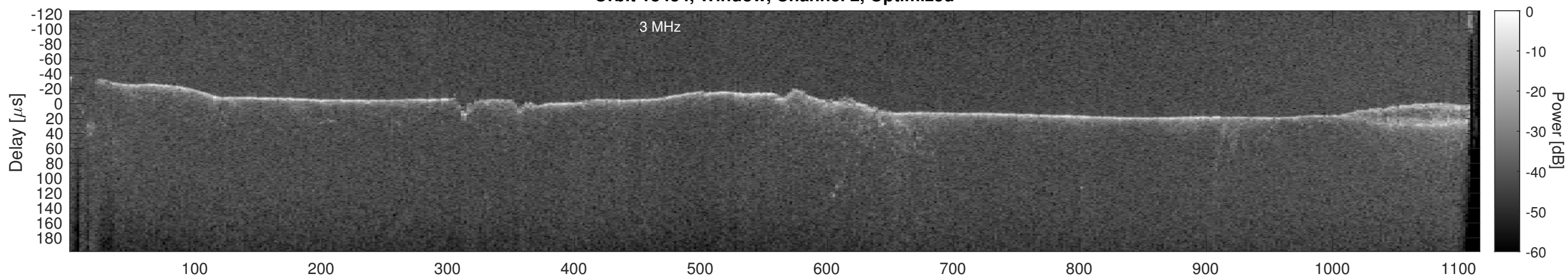
Orbit 18434, Cluttergram
