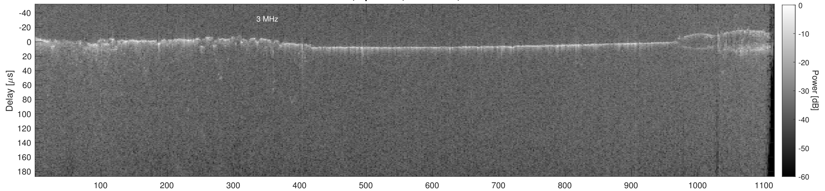
Orbit 18437, Cluttergram
