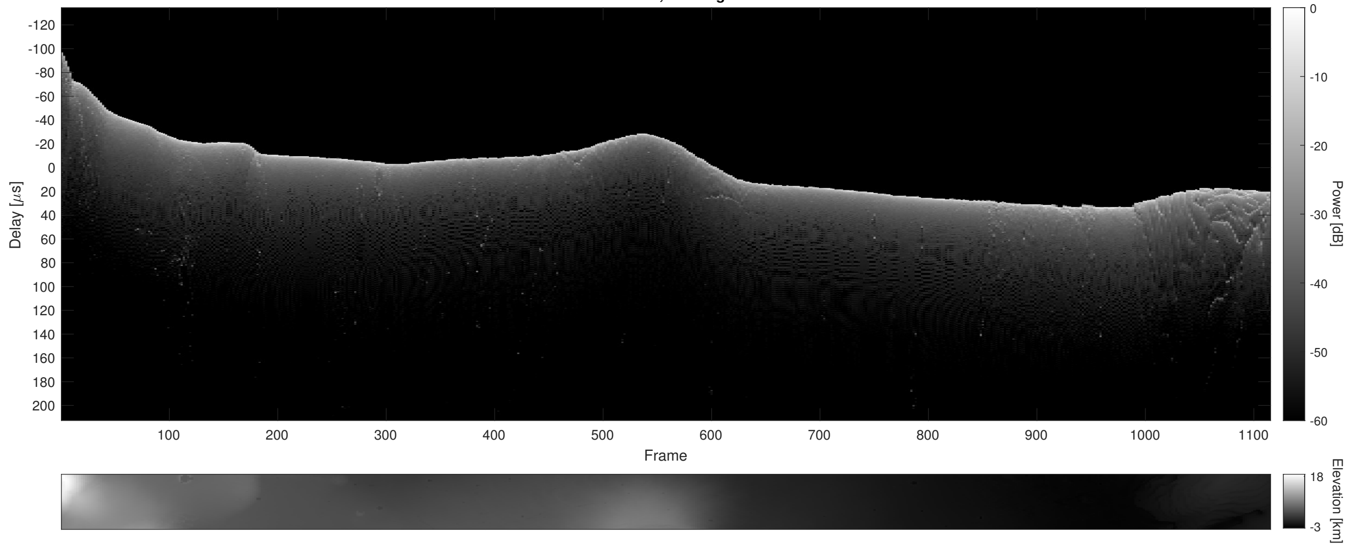
Orbit 18438, Cluttergram
