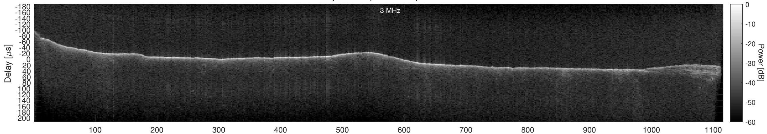
Orbit 18438, Window, Channel 2, Chapman
