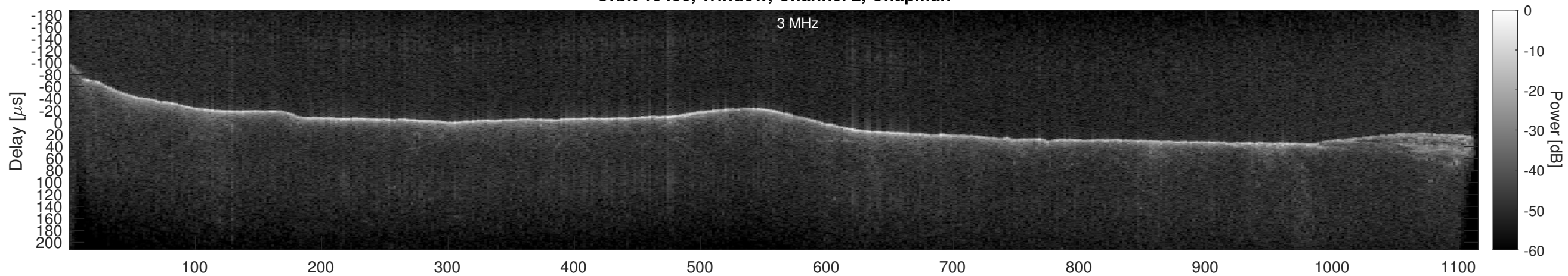
Orbit 18438, Window, Channel 2, Optimized
