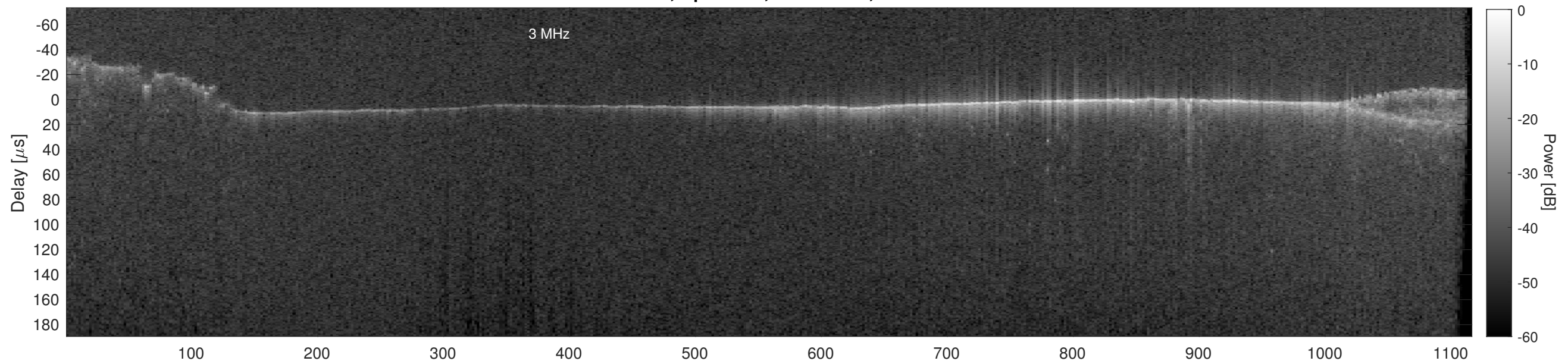
Orbit 18443, Cluttergram
