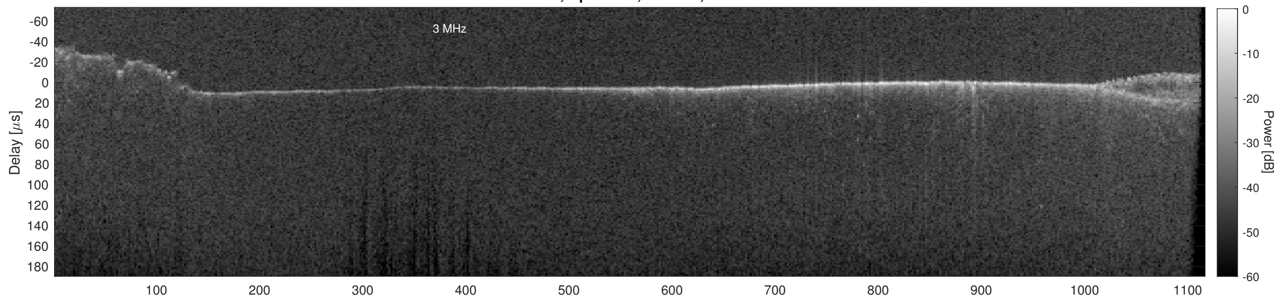
Orbit 18443, Cluttergram
