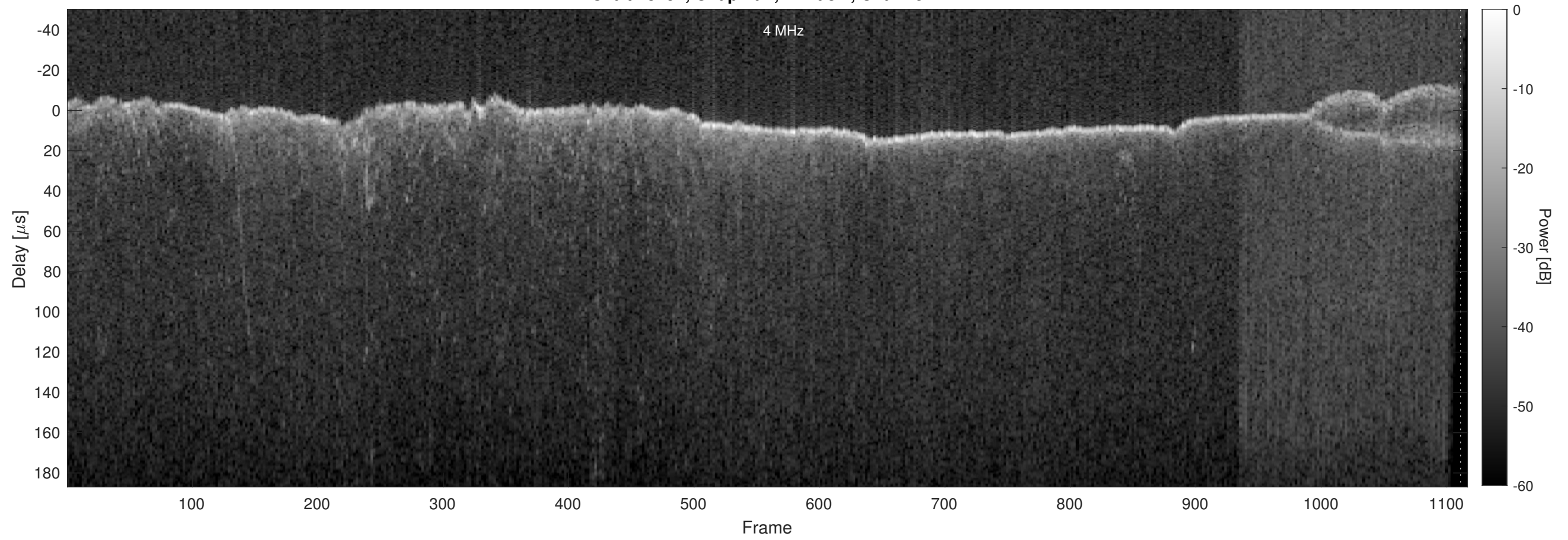
Orbit 18451, Chapman, Window, Channel 2
