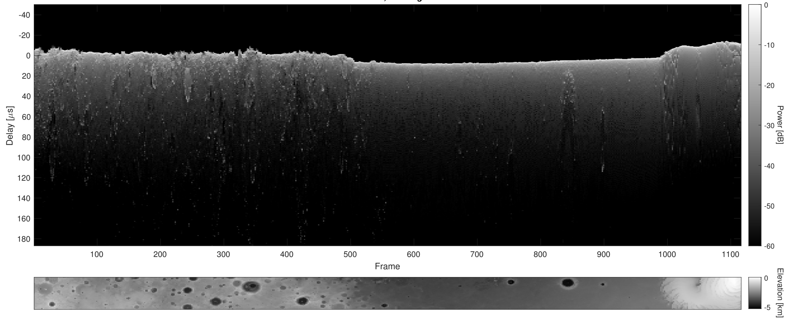
Orbit 18451, Cluttergram
