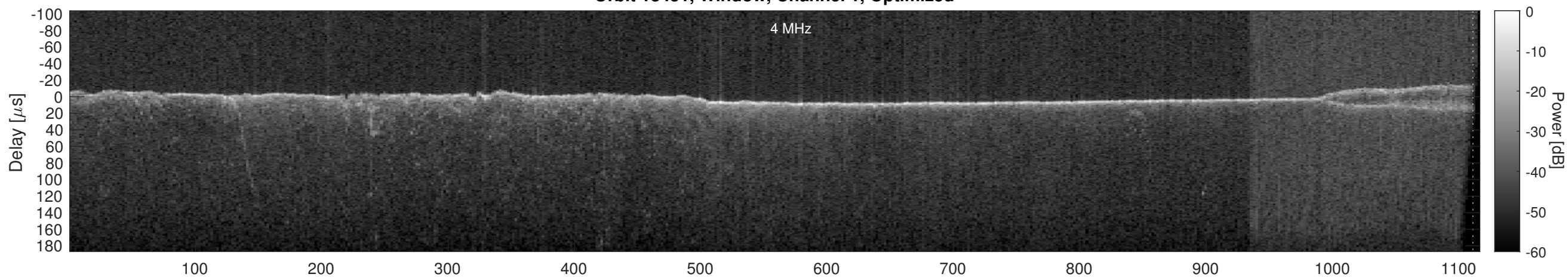
Orbit 18451, Cluttergram
