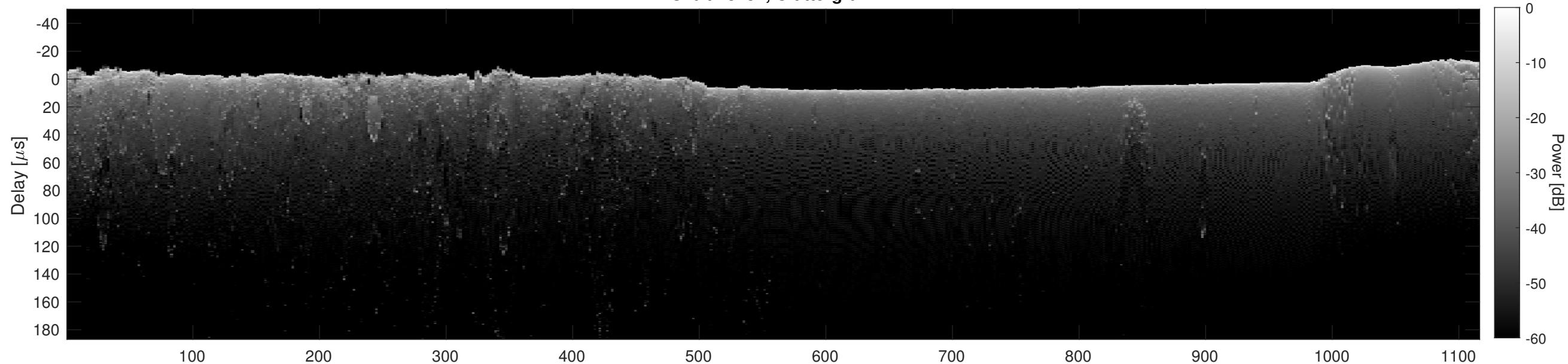
Orbit 18451, Cluttergram
