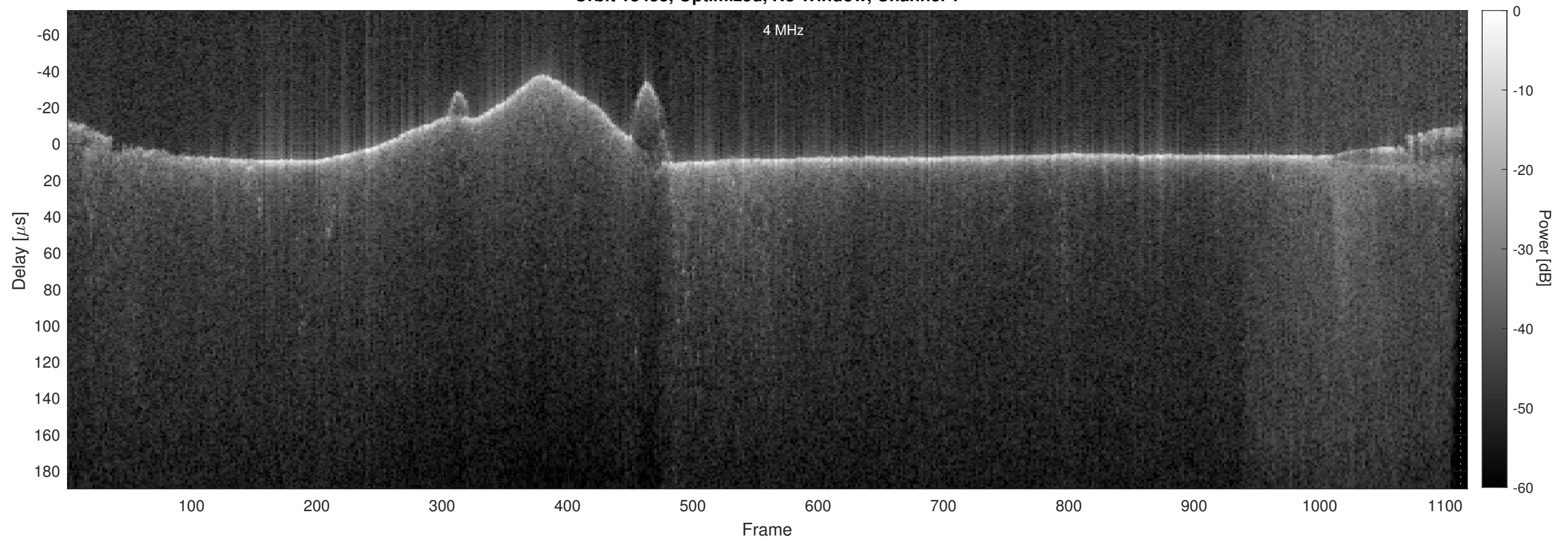
Orbit 18453, Optimized, No Window, Channel 2
