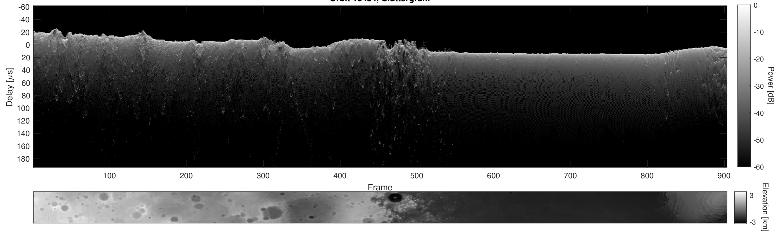
Orbit 18454, Cluttergram
