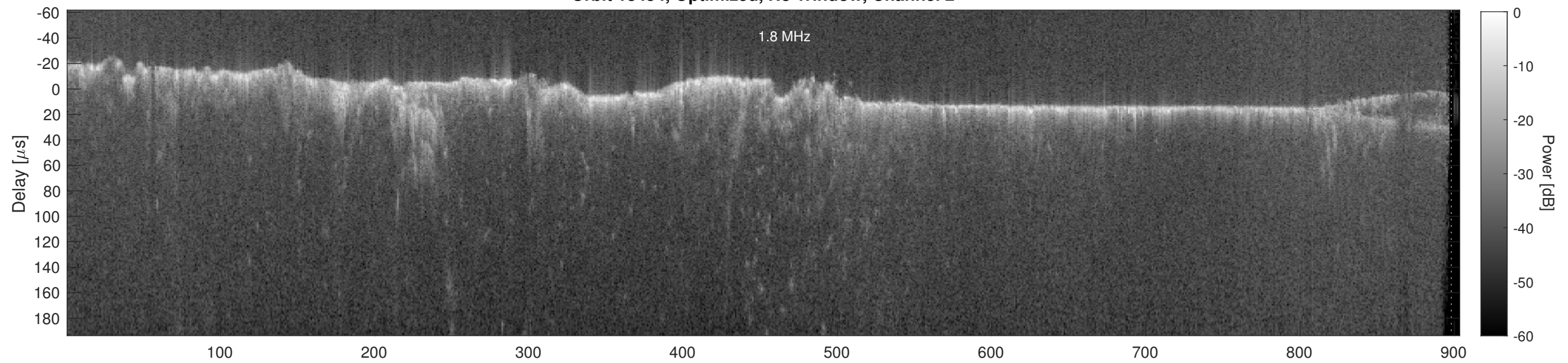
Orbit 18454, Cluttergram
