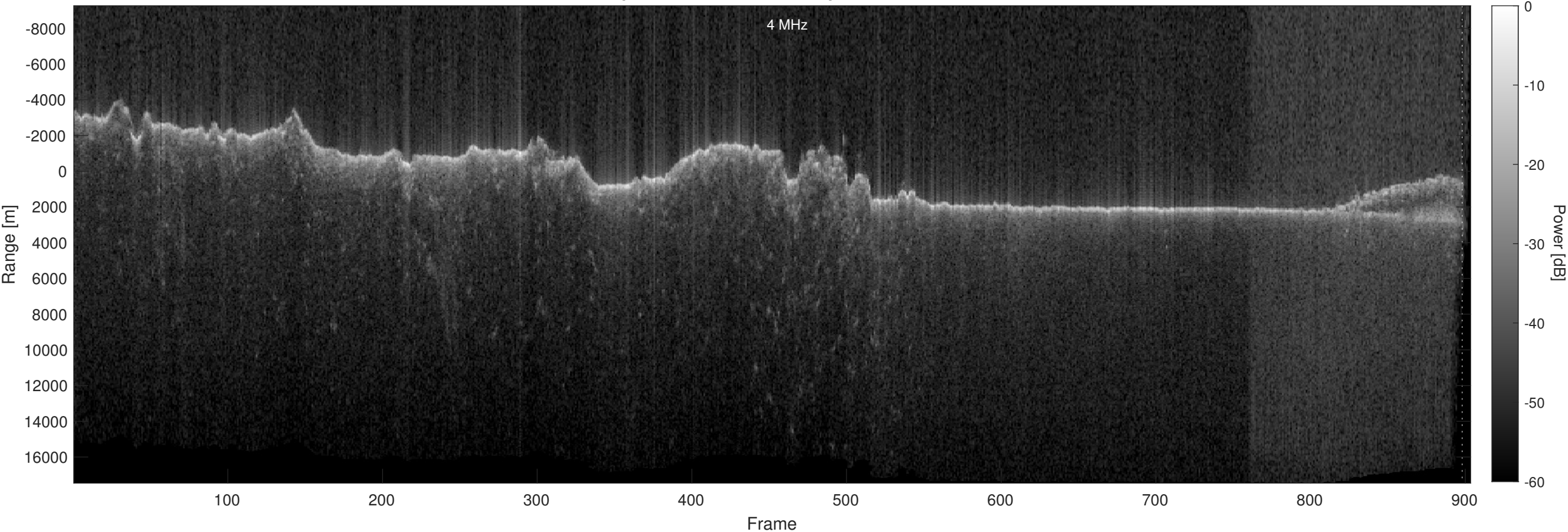
Orbit 18454, Optimized, No Window, Depth-Corrected, Channel 2
