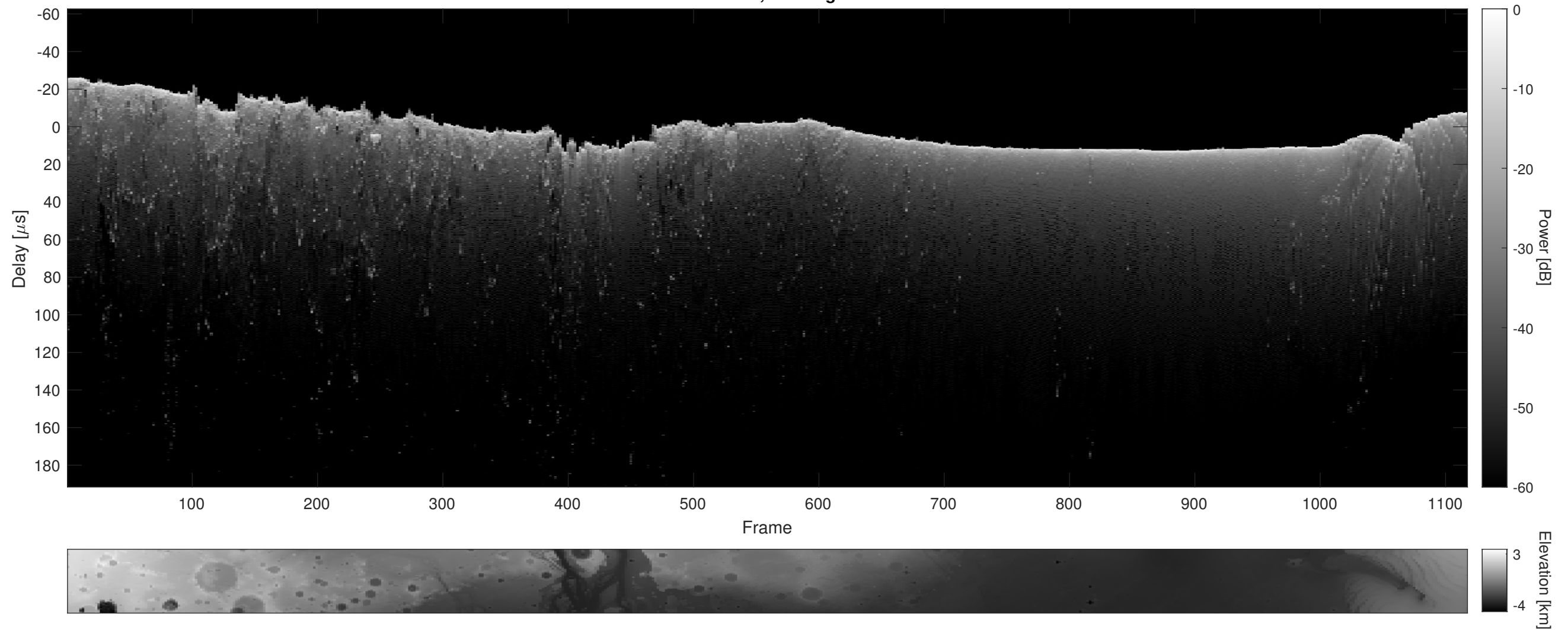
Orbit 18455, Cluttergram
