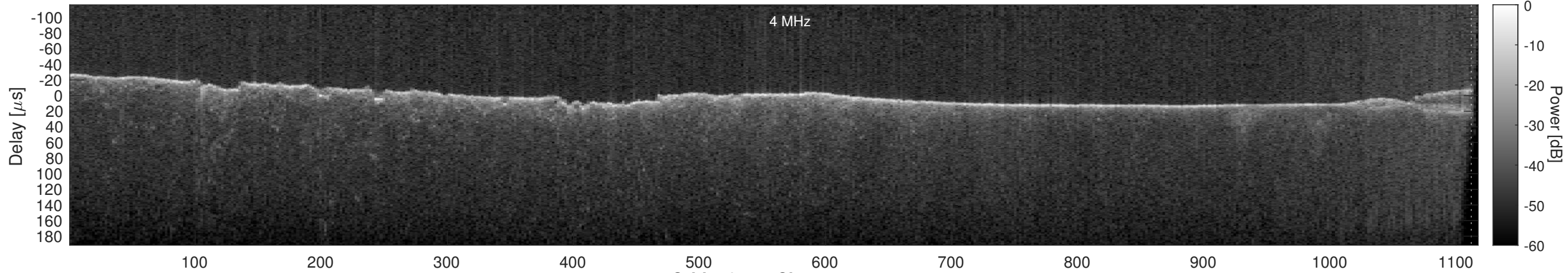
Orbit 18455, Cluttergram
