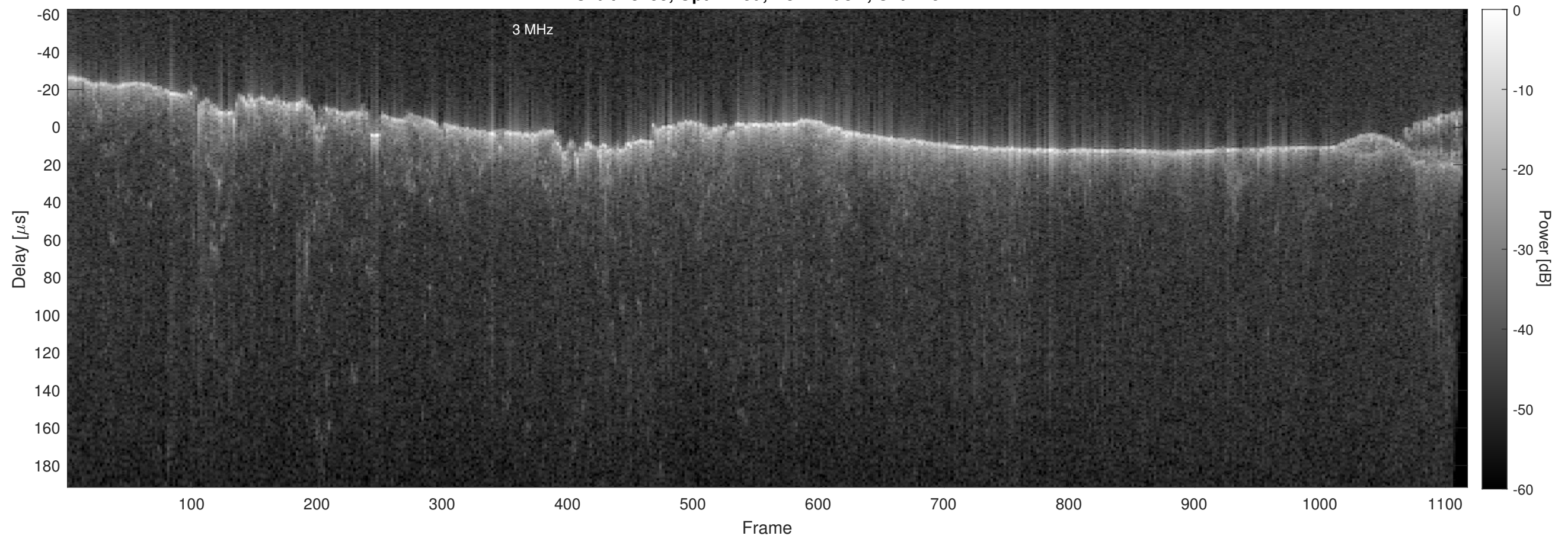
Orbit 18455, Optimized, No Window, Channel 2
