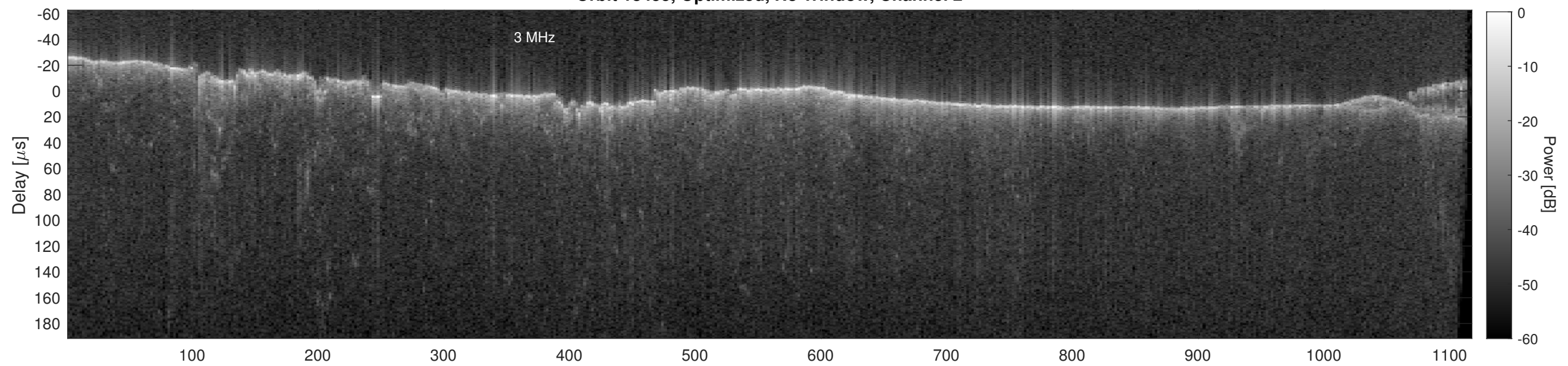
Orbit 18455, Cluttergram
