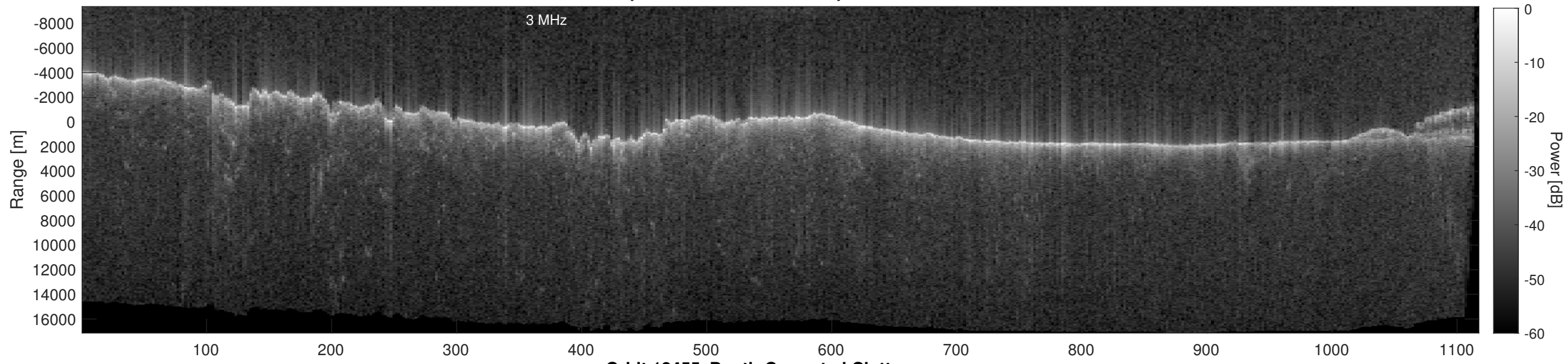
Orbit 18455, Depth-Corrected Cluttergram
