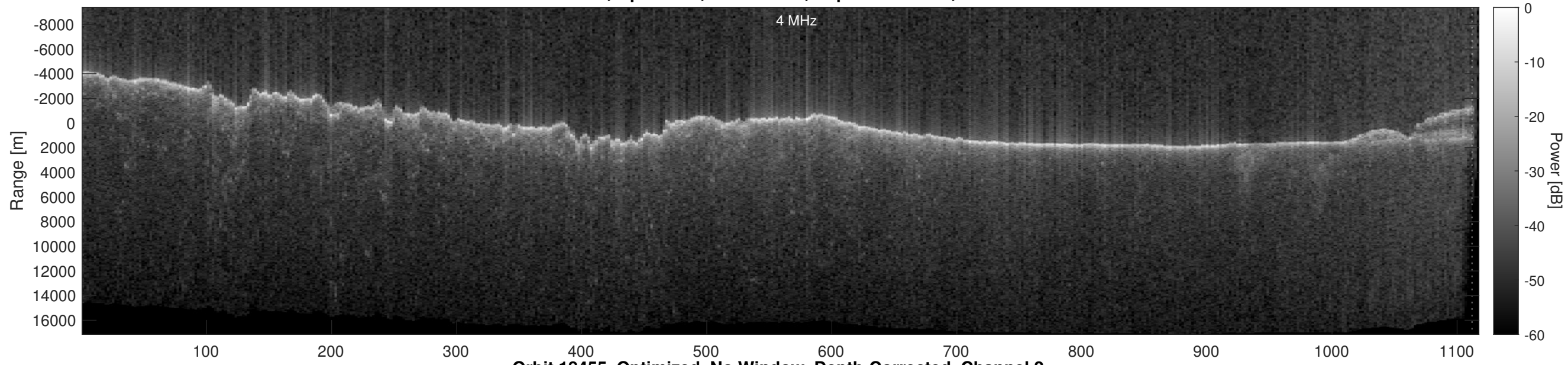
Orbit 18455, Optimized, No Window, Depth-Corrected, Channel 2
