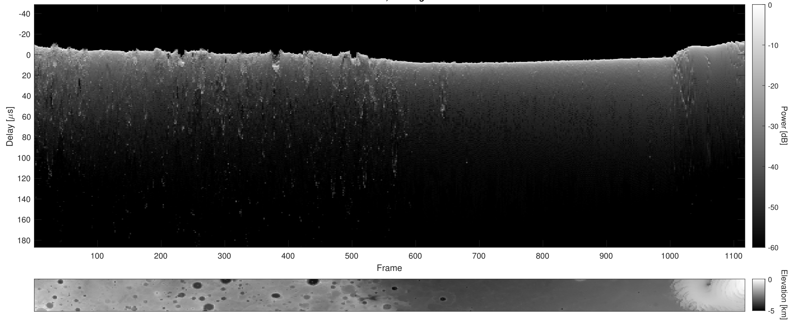
Orbit 18458, Cluttergram
