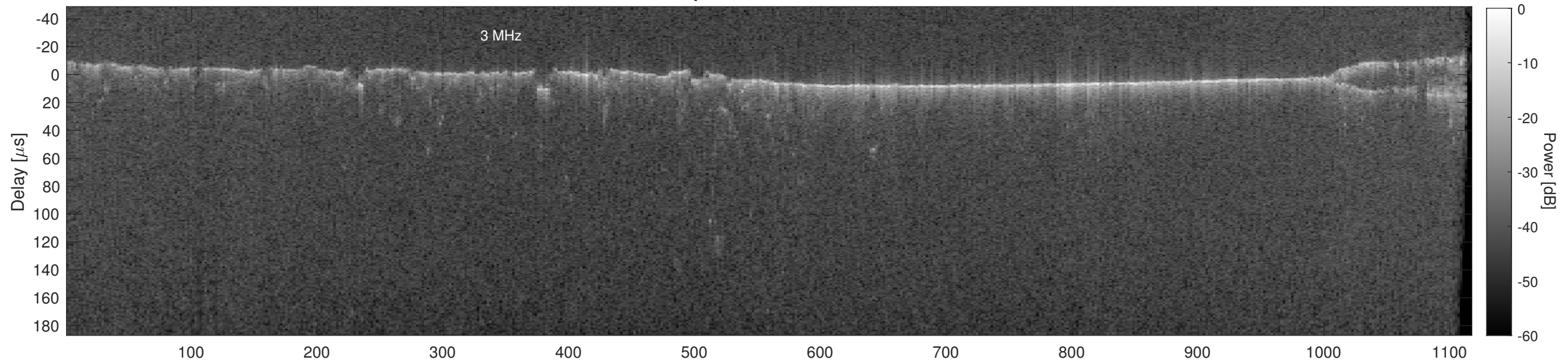
Orbit 18458, Cluttergram
