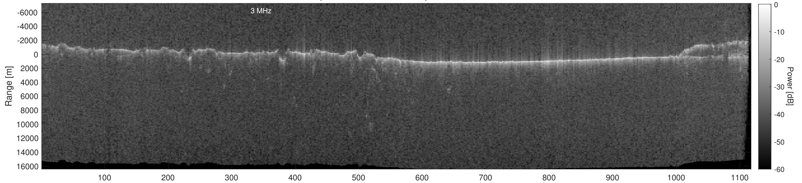
Orbit 18458, Depth-Corrected Cluttergram
